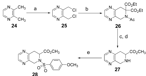
Scheme 4. Reagents: (a) N -chlorosuccinimide, benzoyl peroxide; (b) diethyl acetamidomalonate, \text{Cs}_2\text{CO}_3 ; (c) 6 N HCl; (d) \text{SOCl}_2 , MeOH; (e) 4-methoxybenzenesulfonyl chloride, 4-dimethylaminopyridine.
