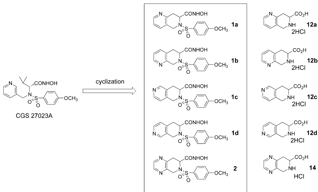
Figure 1. Design of bicyclic compounds from CGS 27023A.
