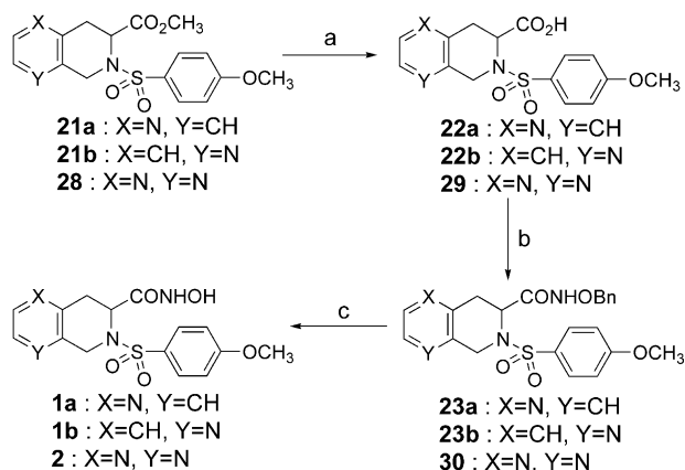
Scheme 3. (Method A). Reagents: (a) NaOH aq; (b) \text{H}_2\text{NOBn}\cdot\text{HCl} , EDCI, HOBt, \text{Et}_3\text{N} ; (c) Pd/C, \text{H}_2 .
