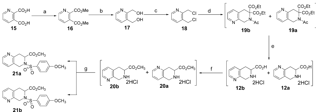
Scheme 2. Reagents: (a) conc \text{H}_2\text{SO}_4 , MeOH; (b) \text{NaBH}_4 ; (c) (i) \text{SOCl}_2 ; (ii) \text{NaHCO}_3 aq; (d) diethyl acetamidomalonate, NaH; (e) 6 N HCl; (f) \text{SOCl}_2 , MeOH; (g) 4-methoxybenzenesulfonyl chloride, 4-dimethylaminopyridine.
