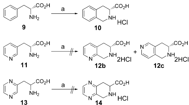
Scheme 1. Reagents: (a) formaldehyde, hydrochloric acid.
