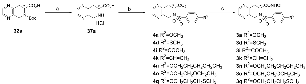
Scheme 7. (Method C). Reagents: (a) 4 N \text{HCl} /ethyl acetate solution; (b) 4-substituted benzenesulfonyl chloride; (c) (i) \text{ClCOCOCl} , (ii) \text{H}_2\text{NOH} aq.
