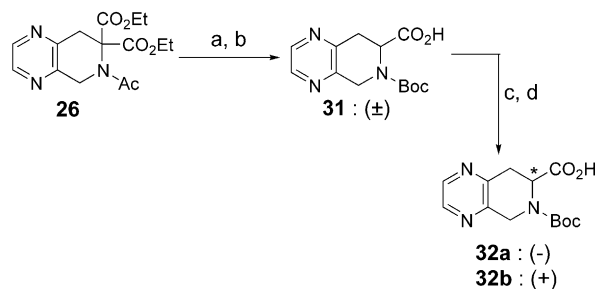
Scheme 5. Reagents: (a) 6 N HCl; (b) di- tert -dicarbonate, NaOH; (c) ( S )-(-)-1-phenylethylamine or ( R )-(+)-1-phenylethylamine; (d) citric acid.
